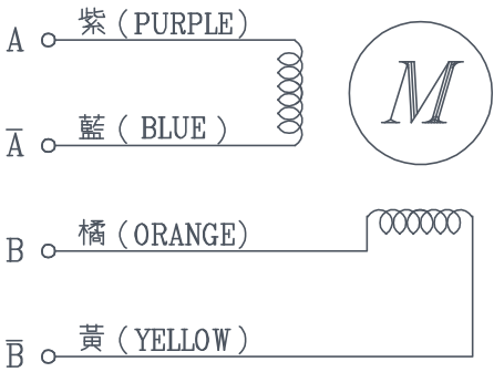
齒輪箱馬達接線圖/ Geared Motor Wiring Diagram
