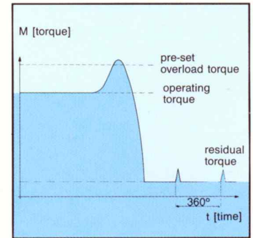
Switching behaviour
