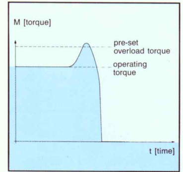
Switching behaviour
