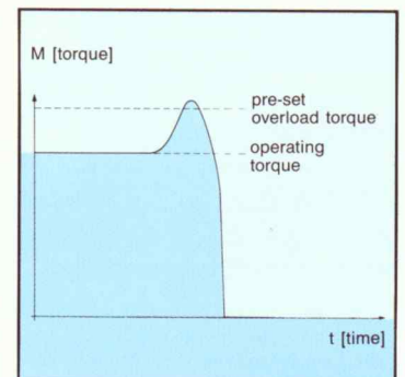
Switching behaviour
